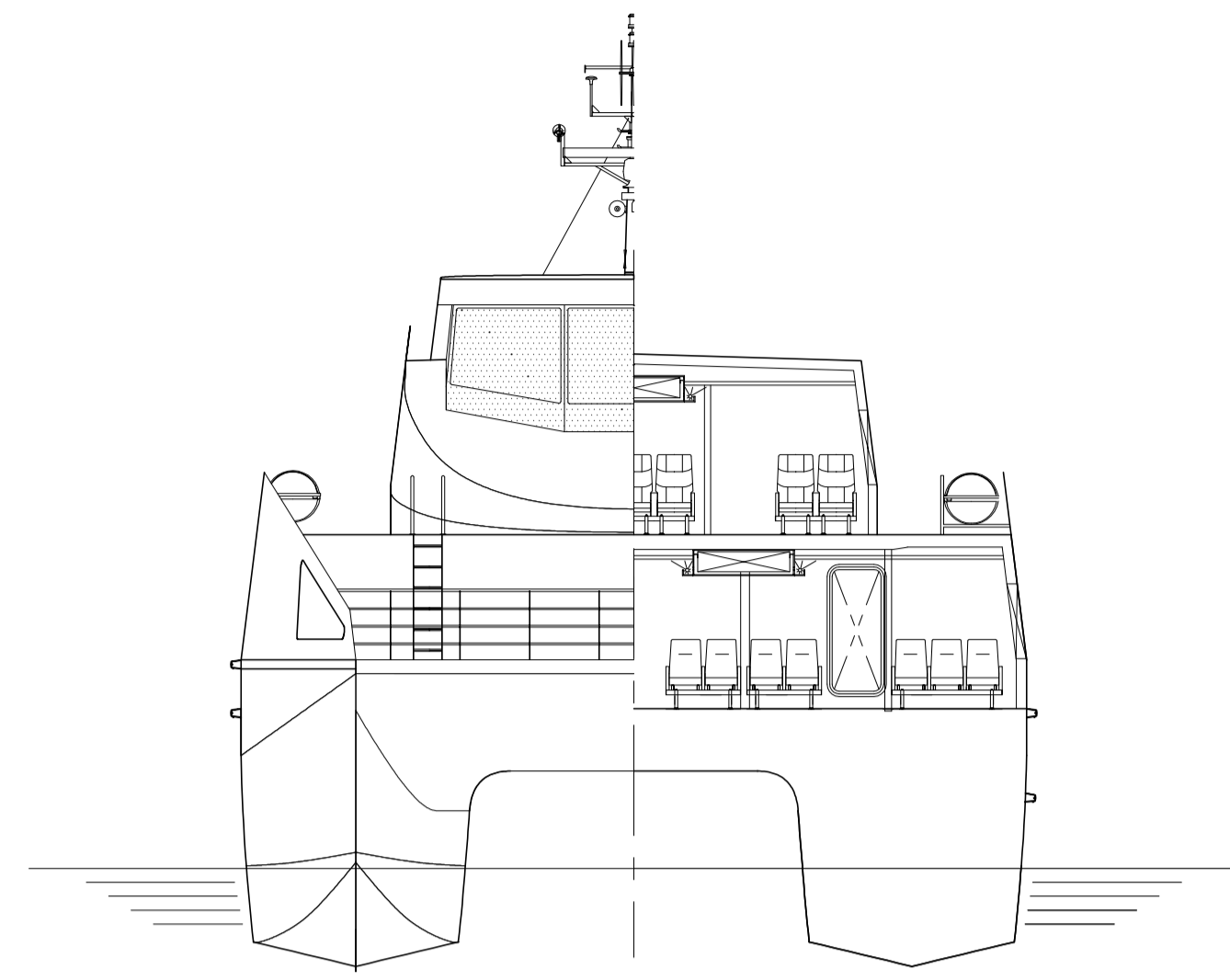
Bow view
