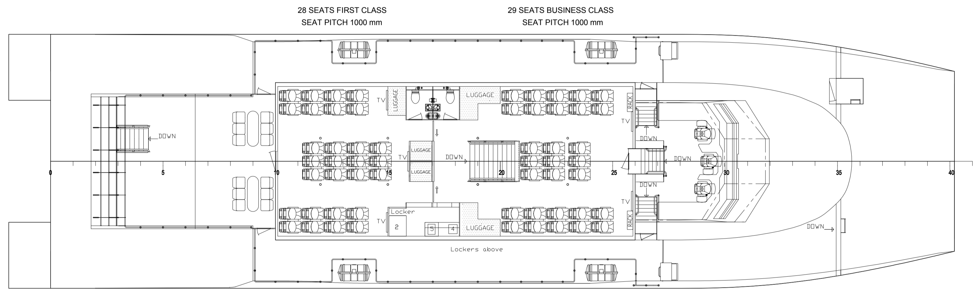
Upper deck
