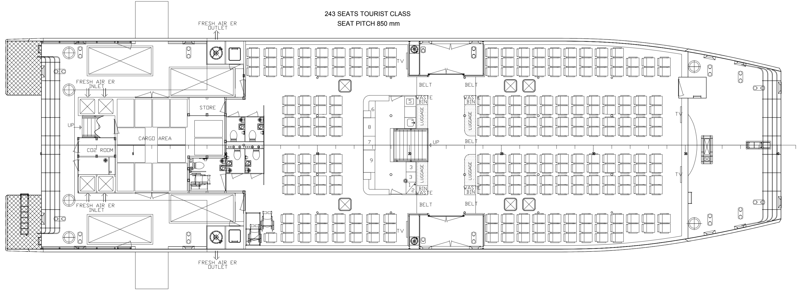
Main deck
